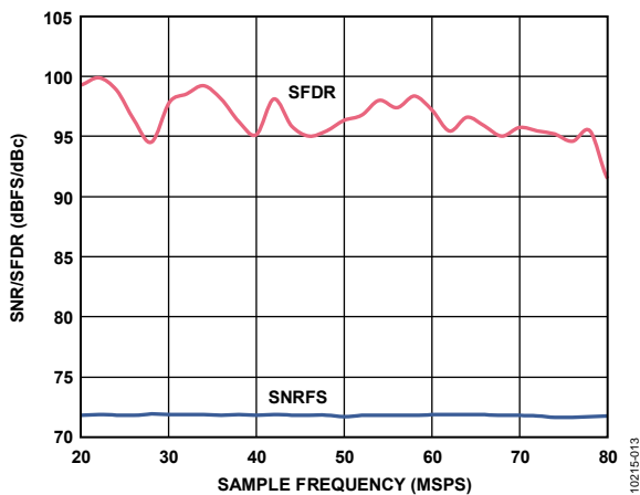
Figure 14. SNR/SFDR vs. Encode, f_{IN} = 19.7 MHz
